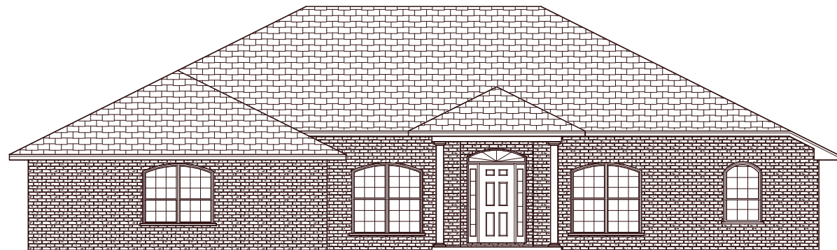
* FRONT ELEVATION *
